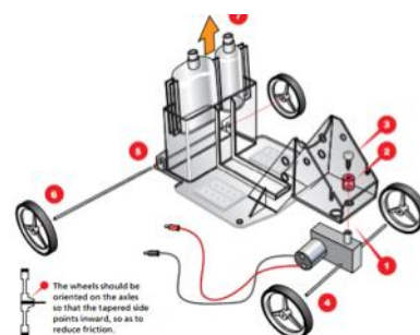
Figure 1: Car Assembly
