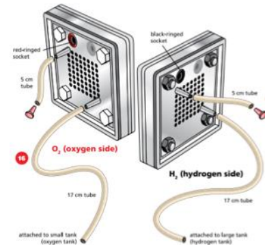
Figure 3: Fuel Cell Assembly
